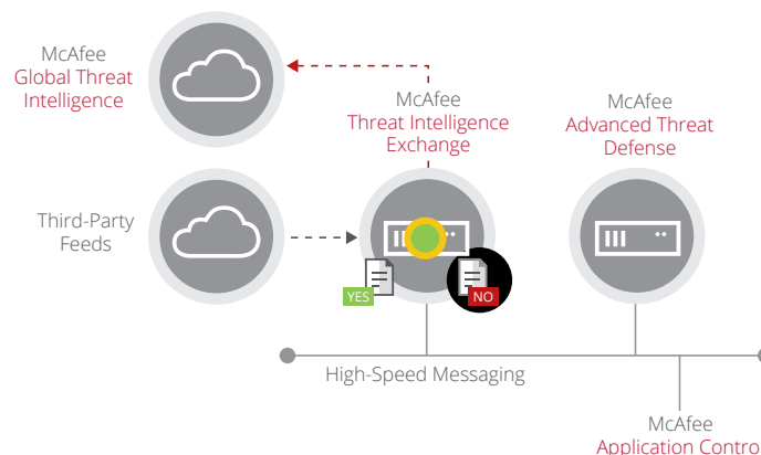
Figure 2. McAfee GTI constantly monitors the reputation of files and senders. When deployed with McAfee Threat Intelligence Exchange, McAfee Application Control automatically updates the whitelist based on local reputation intelligence and can coordinate with McAfee Advanced Threat Defense if more information on a file is needed.
